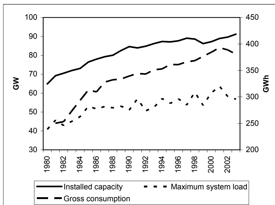
Figure 6: Capacity, consumption and system load (source: Nordel)
